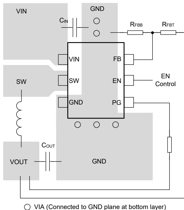
图 8-26. Suggested Layout
