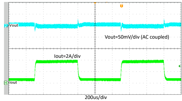
图 8-17. TPS564255 Transient Response with 0.4 A to 3.6 A
