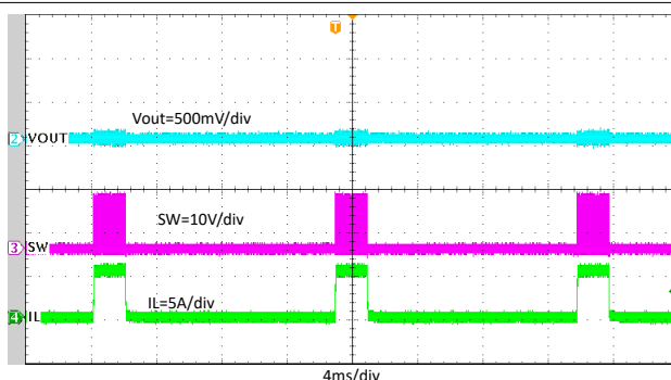
图 8-25. Output Hard Short Hiccup
