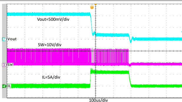
图 8-23. TPS564257 Normal Operation to Output Hard Short
