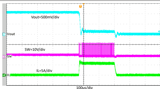
图 8-22. TPS564252 Normal Operation to Output Hard Short
