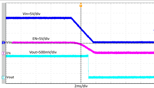
图 8-21. Shutdown with V_{IN} Falling, I_{OUT} = 4\text{ A}
