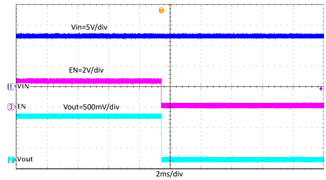
图 8-19. Shutdown Through EN, I_{OUT} = 4\text{ A}
