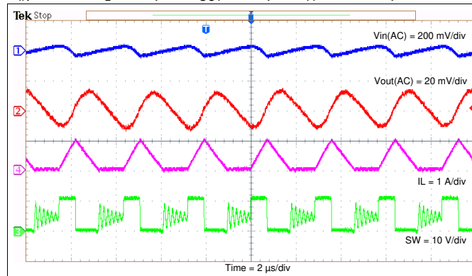
图 24. Steady State Waveforms, I_{OUT} = 0.3\text{ A}
