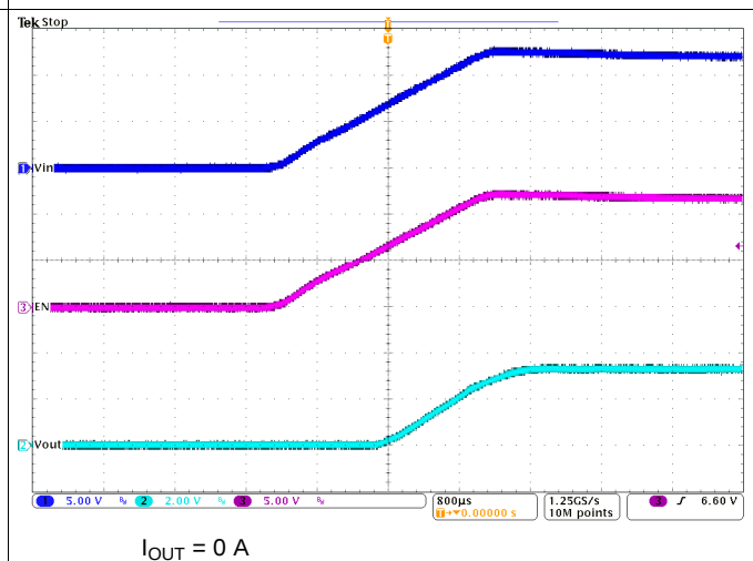
图 31. Start Up Relative to V_{IN}
