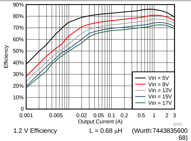
图 12. Efficiency vs Output Current, V_{OUT} = 1.2\text{ V}
