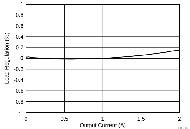
图 21. TPS562219A Load Regulation, V_I = 12\text{ V}
