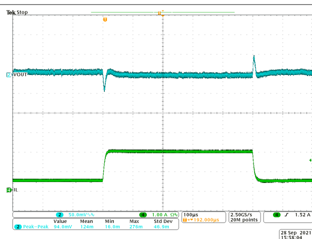
图 8-11. Transient Response 0.5 to 2 A with Slew Rate of 2.5\text{ A}/\mu\text{s}
