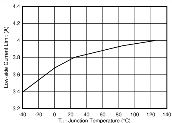
图 6-10. Low-Side Current Limit Threshold vs Junction Temperature
