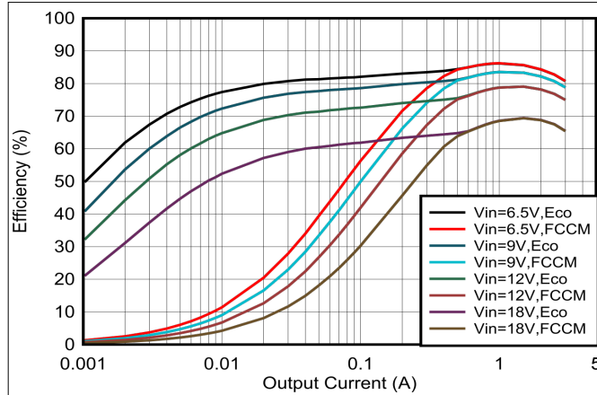
图 6-13. V_{OUT} = 1.05\text{-V} Efficiency, L = 0.68\text{ }\mu\text{H}
