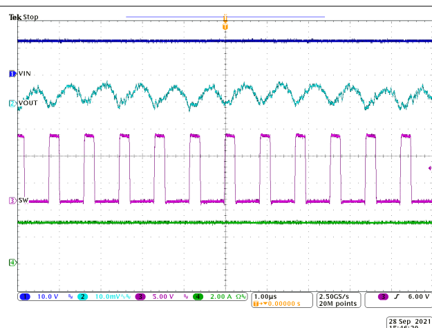
图 8-9. Steady State Waveforms, I_{OUT} = 3\text{ A}
