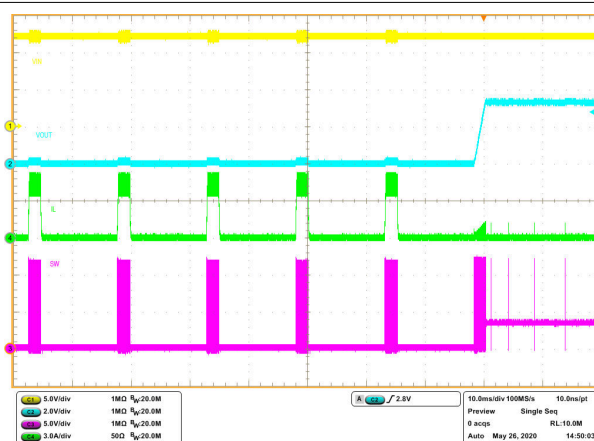
图 8-19. Output Short Recovery (ECO)
