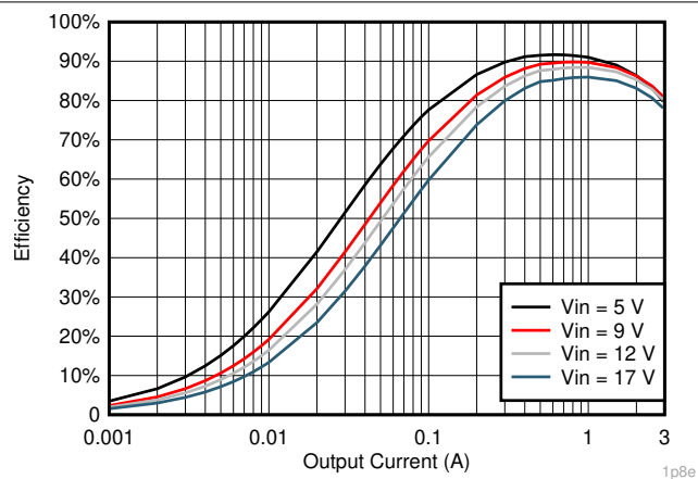
图 7-12. V_{OUT} = 1.8V 效率, L = 2.2\mu H
