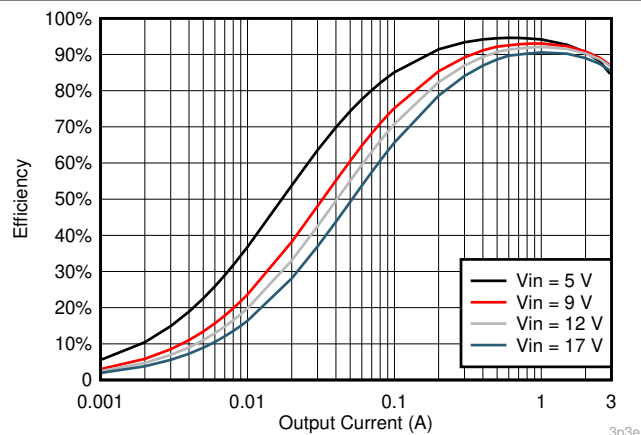
图 7-13. V_{OUT} = 3.3V 效率, L = 3.3\mu H
