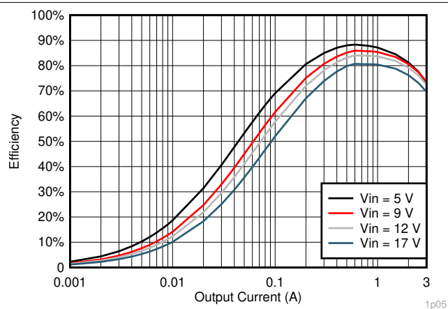
图 7-10. V_{OUT} = 1.05V 效率, L = 1.5\mu H
