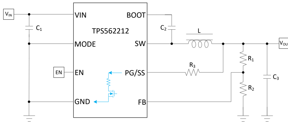
图 7-2. Discharge VOUT Through PG/SS Pin with TPS562212
