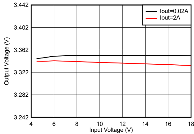
图 8-4. Line Regulation
