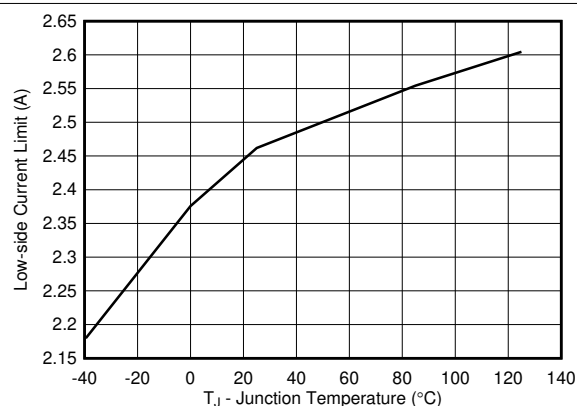
图 6-10. Low-Side Current Limit Threshold vs Junction Temperature
