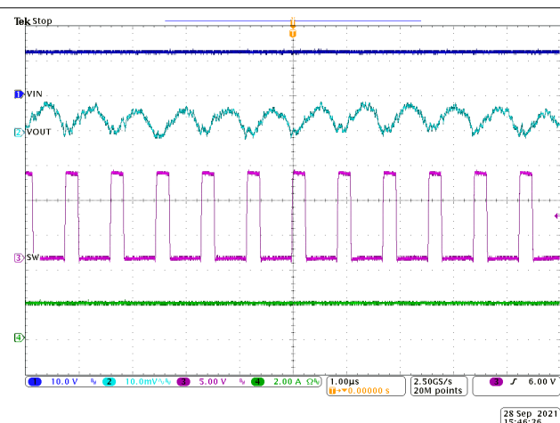
图 8-9. Steady State Waveforms, I_{OUT} = 2\text{ A}
