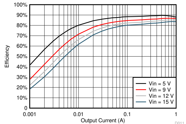
图 6-10. TPS561201 V_{OUT} = 1.5 V, Efficiency, L = 2.2 \mu H
