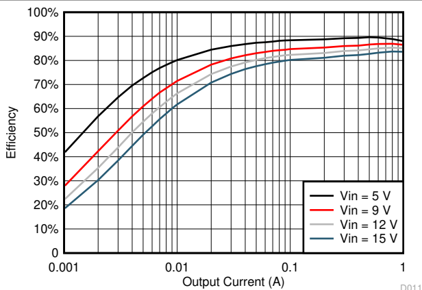
图 6-10. TPS561201 V_{OUT} = 1.5 V, Efficiency, L = 2.2 \mu H
