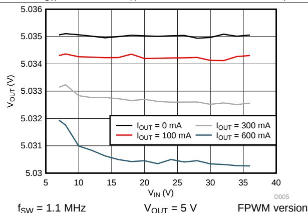
图 7. Line Regulation
