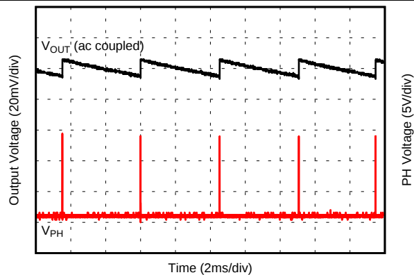
图 18. Output Ripple, I_{OUT} = 0 mA
