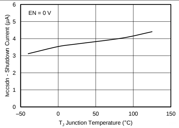
图 2. Shutdown Current vs Junction Temperature
