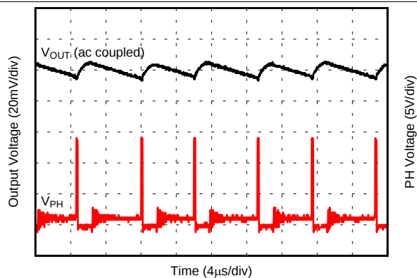
图 17. Output Ripple, I_{OUT} = 30 mA
