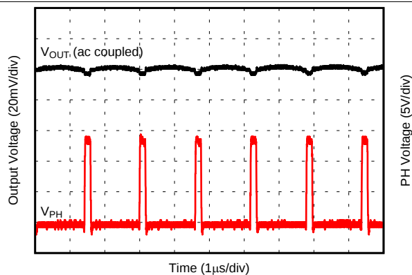
图 16. Output Ripple, I_{OUT} = 500 mA
