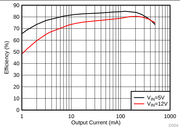
图 9. Light-Load Efficiency
