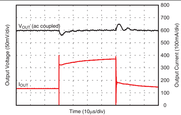
图 13. Transient Response, 25% to 75% Load Step
