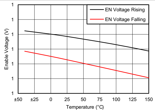
图 6-12. Enable Voltage vs Temperature
