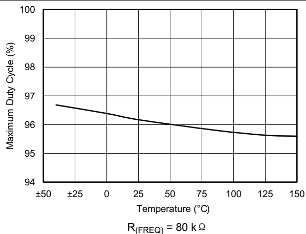
图 6-13. Maximum Duty Cycle vs Temperature
