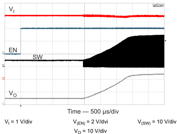
图 8-8. Start-Up
