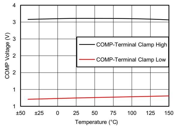
图 6-10. COMP Clamp Voltage vs Temperature
