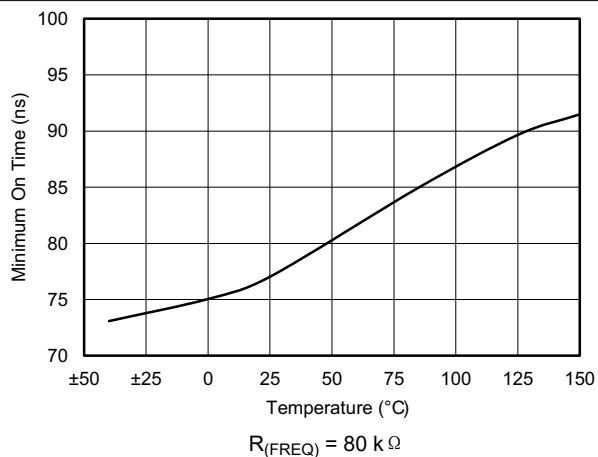
图 6-14. Minimum On Time vs Temperature
