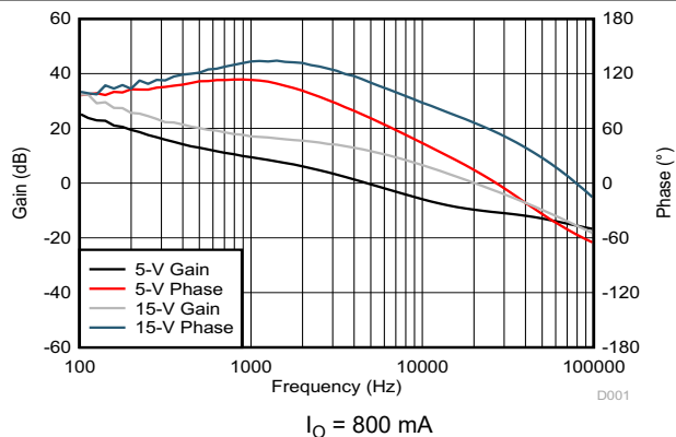
图 8-9. Closed Loop Gain and Phase of the Boost Converter
