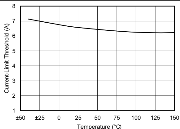
图 6-2. Switch Current Limit vs Temperature
