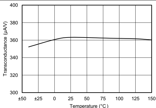
图 6-1. Error Amplifier Transconductance vs Temperature
