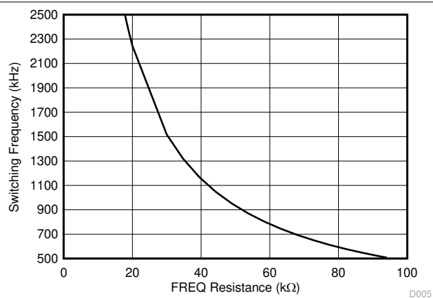
图 6-6. Frequency vs FREQ Resistance High Frequency Range
