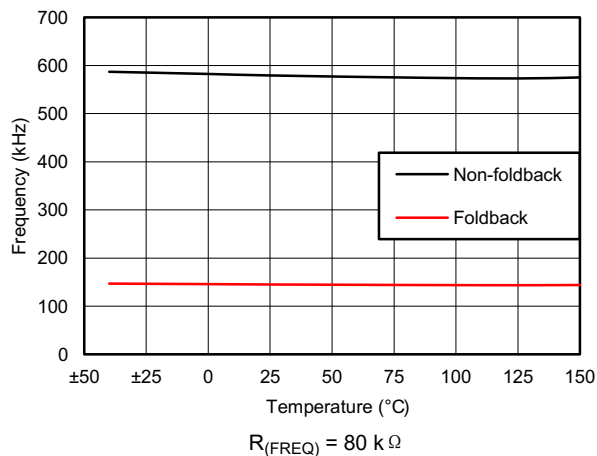
图 6-9. Non-Foldback Frequency vs Foldback Frequency
