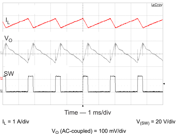
图 8-5. CCM PWM Operation
