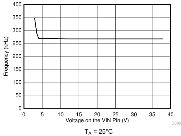
图 6-7. Minimum Switching Frequency for Quick Recovery from Frequency Foldback
