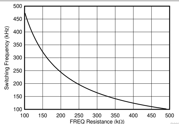
图 6-5. Frequency vs FREQ Resistance Low Frequency Range
