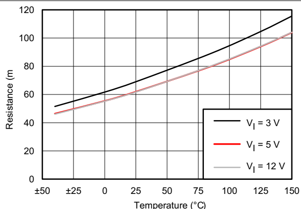
图 6-4. Static Drain Source On-State Resistance ( r_{\text{DS(on)}} ) vs Temperature
