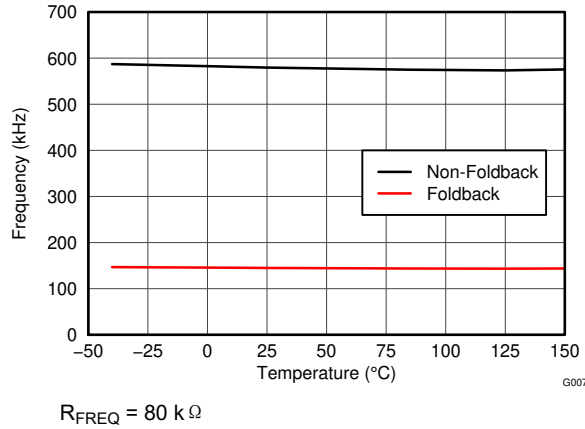
图 7-7. Non-Foldback Frequency vs Foldback Frequency
