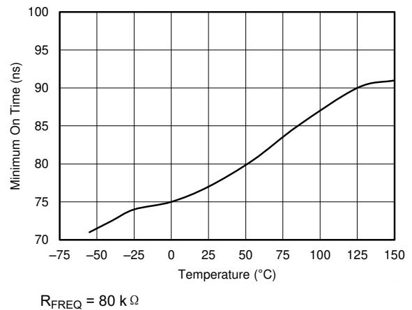
图 7-12. Minimum On Time vs Temperature
