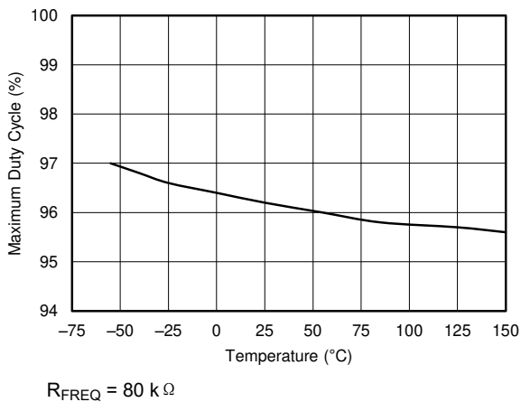
图 7-11. Maximum Duty Cycle vs Temperature
