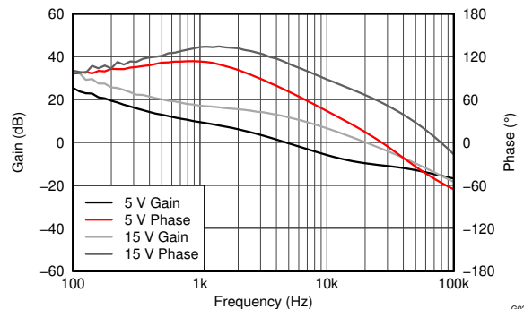
图 9-9. Closed Loop Gain and Phase of the Boost Converter
