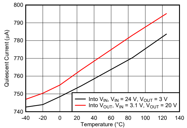
图 6-16. Quiescent Current vs Temperature
