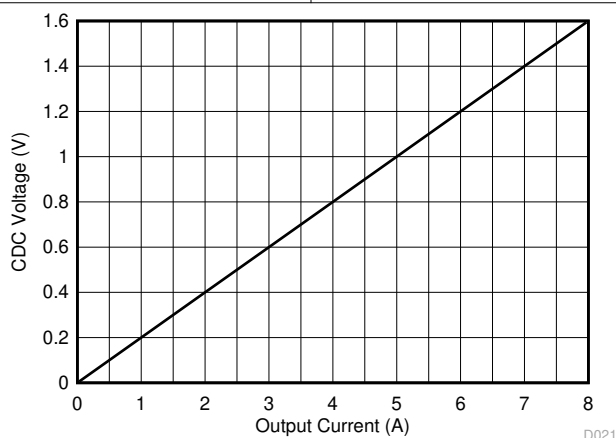
图 6-21. CDC Voltage vs Output Current with R_{\text{SENSE}} = 10 \text{ m}\Omega
