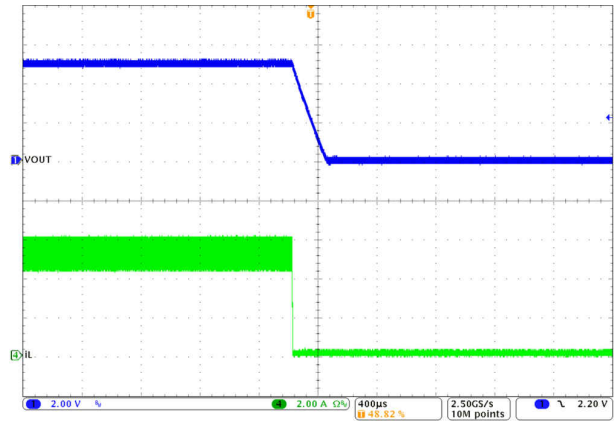
图 8-9. Shutdown Waveforms in V_{IN} = 12\text{ V} , V_{OUT} = 5\text{ V} , I_{OUT} = 5\text{ A} , FPWM
