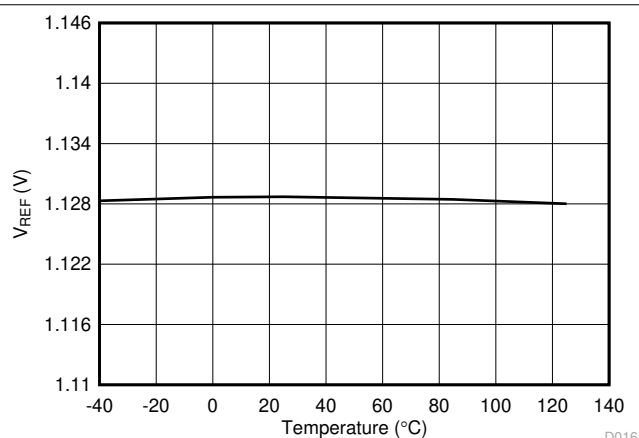
图 6-16. Reference Voltage vs Temperature ( V_{REF} = 1.129 V)
