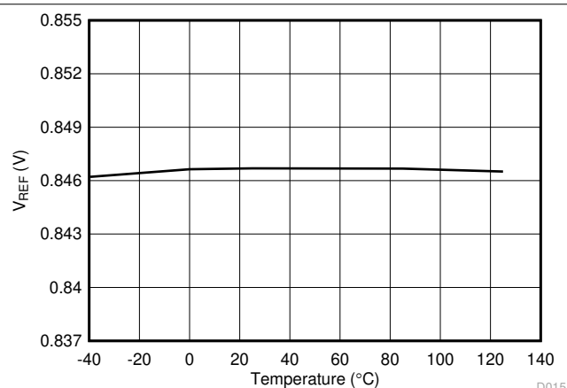
图 6-15. Reference Voltage vs Temperature ( V_{REF} = 0.846 V)
