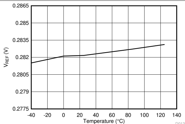
图 6-13. Reference Voltage vs Temperature ( V_{REF} = 0.282 V)
