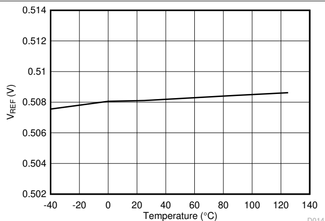
图 6-14. Reference Voltage vs Temperature ( V_{REF} = 0.508 V)
