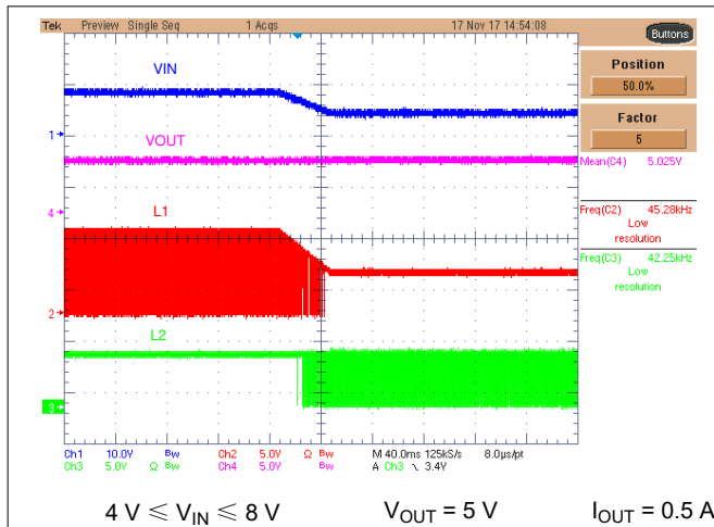
图 7-13. Step-Down to Step-Up Mode Transition
