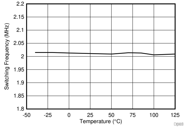
图 7-2. Switching Frequency vs Temperature
