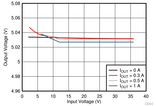
图 7-4. 5-V Output Regulation vs Input Voltage
