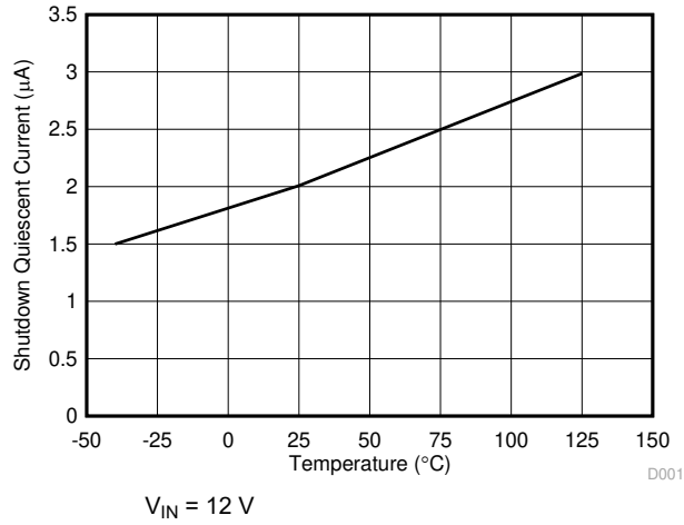
图 7-1. Shutdown I_{\text{Q}} vs Temperature
