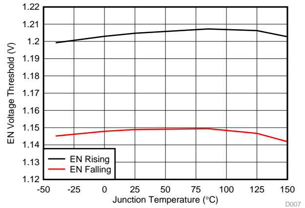
图 8. EN Pin Voltage Threshold vs Junction Temperature
