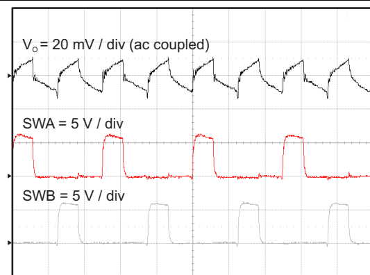
图 57. Full Load Output Voltage Ripple
