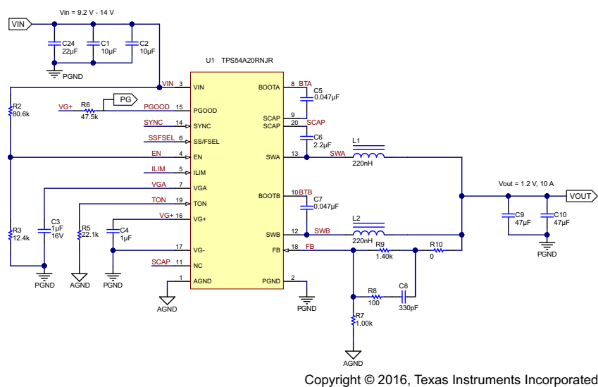
图 47. Typical Application
