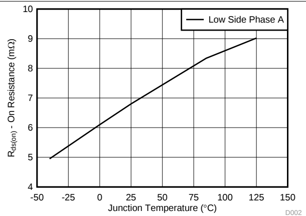
图 2. On Resistance vs Junction Temperature
