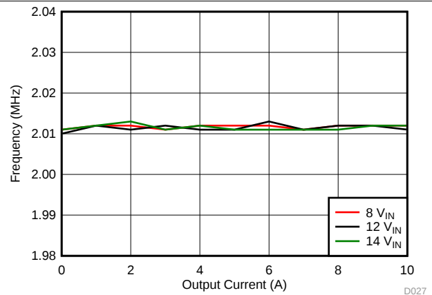
图 26. Frequency vs Output Current
