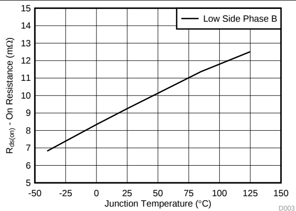
图 1. On Resistance vs Junction Temperature
