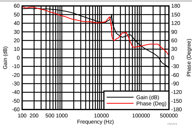
图 52. Loop Response
