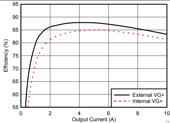
图 19. Efficiency vs Output Current for Gate Drive Supply
