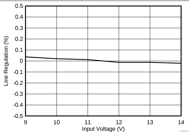
图 51. Line Regulation
