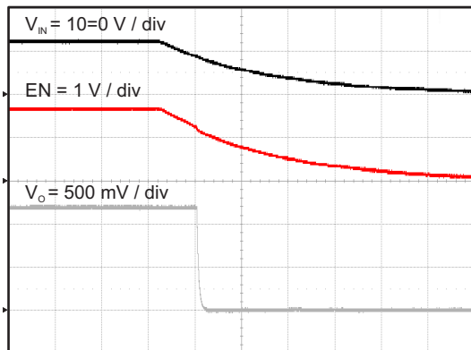
Time = 2 msec / div 图 60. Shut Down with VIN
