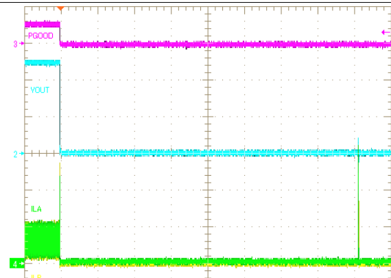
图 34. Shutdown Through VIN
