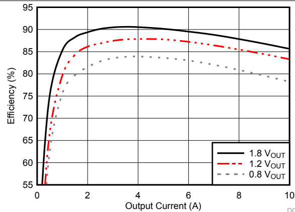
图 20. Efficiency vs Output Current for Output Voltage
