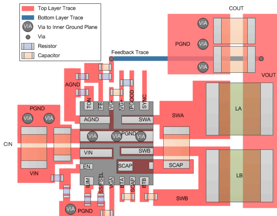
图 62. Layout Recommendation
