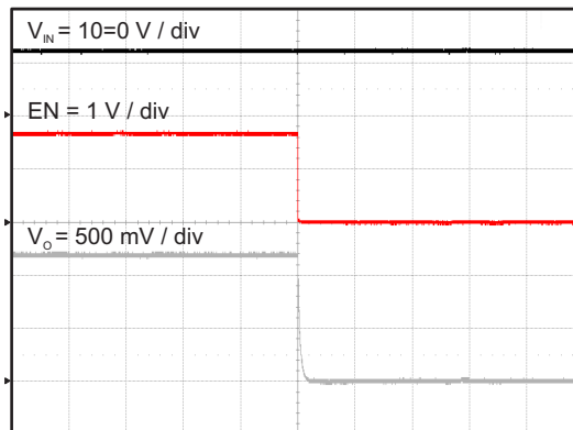
Time = 2 msec / div 图 61. Shut Down with EN
