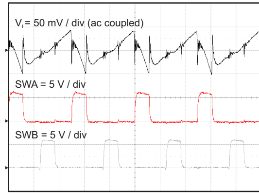
图 55. Full Load Input Voltage Ripple
