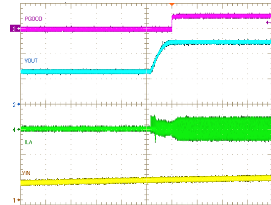
图 32. Pre-biased Startup Through VIN
