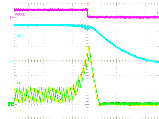
图 33. Shutdown Through VIN
