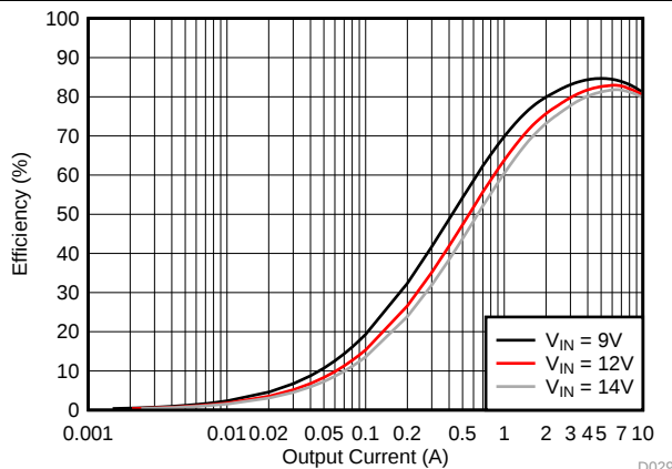
图 49. Light Load Efficiency
