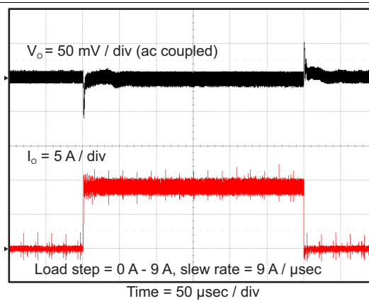
图 53. Transient Response
