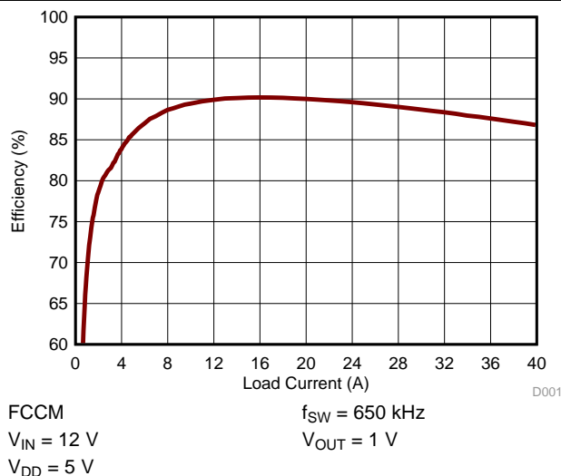
Figure 56. Efficiency vs. Load Current
