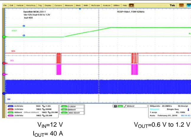
Figure 60. VOUT Command: 0.6 V to 1.2 V, IOUT = 40 A
