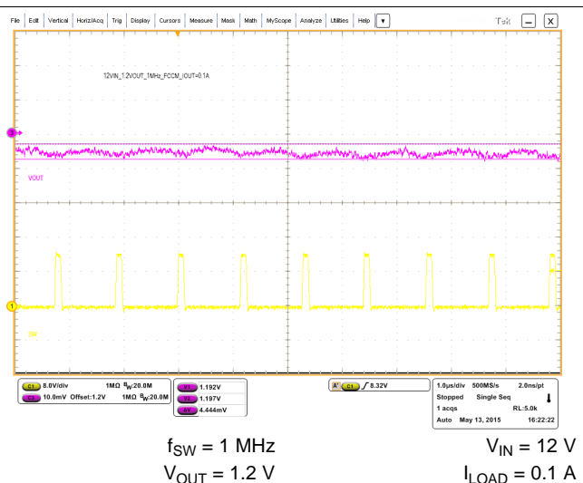
图 15. Steady-State Operation
