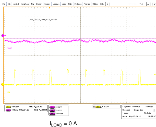
Figure 49. FCCM Steady-State Operation
