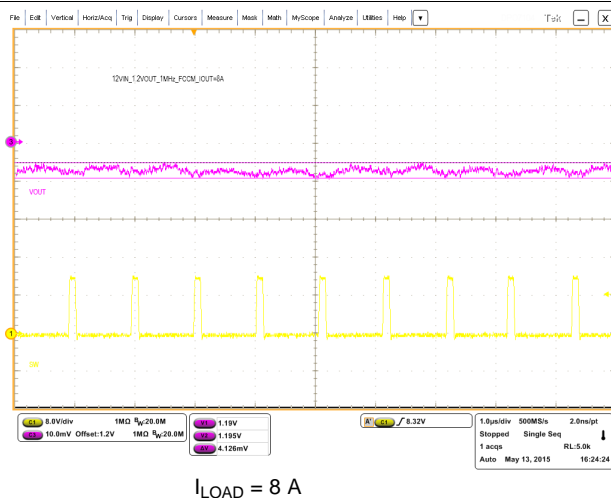
Figure 51. Steady-State Operation
