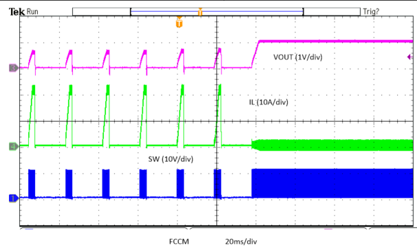
图 8-30. Hiccup Overcurrent
