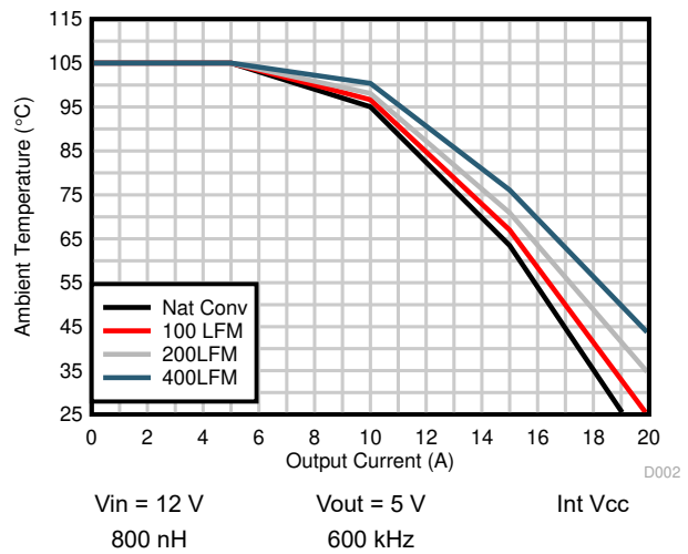
图 6-6. Safe Operating Area, V OUT = 5 V
