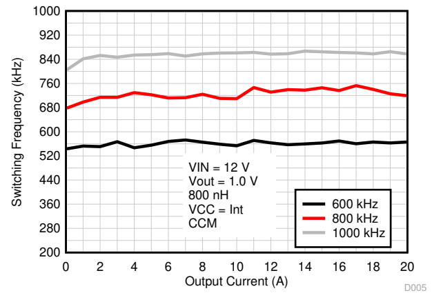
图 8-5. Switching Frequency vs Output Current
