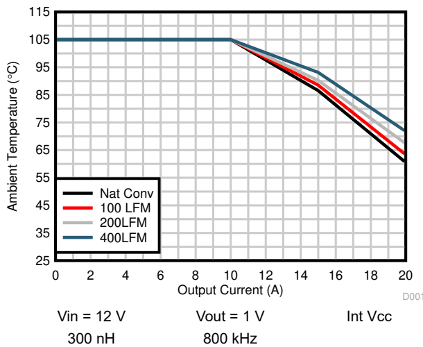
图 6-5. Safe Operating Area, V OUT = 1.0 V
