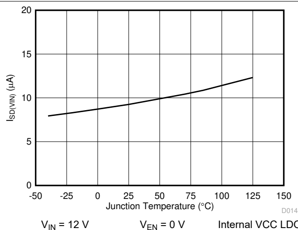
图 6-11. I_{SD(VIN)} vs Junction Temperature
