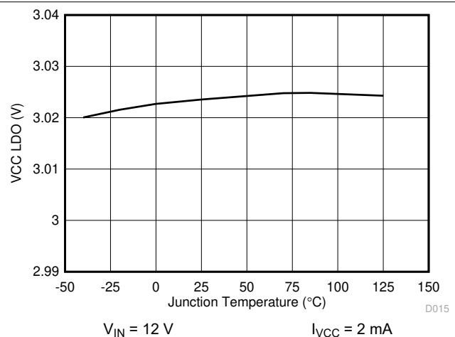
图 6-12. VCC LDO vs Junction Temperature
