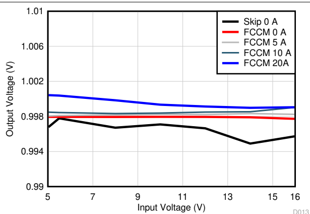
图 8-11. Output Voltage vs Input Voltage VCC = Int
