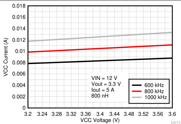
图 8-13. ICC Current vs External VCC Voltage
