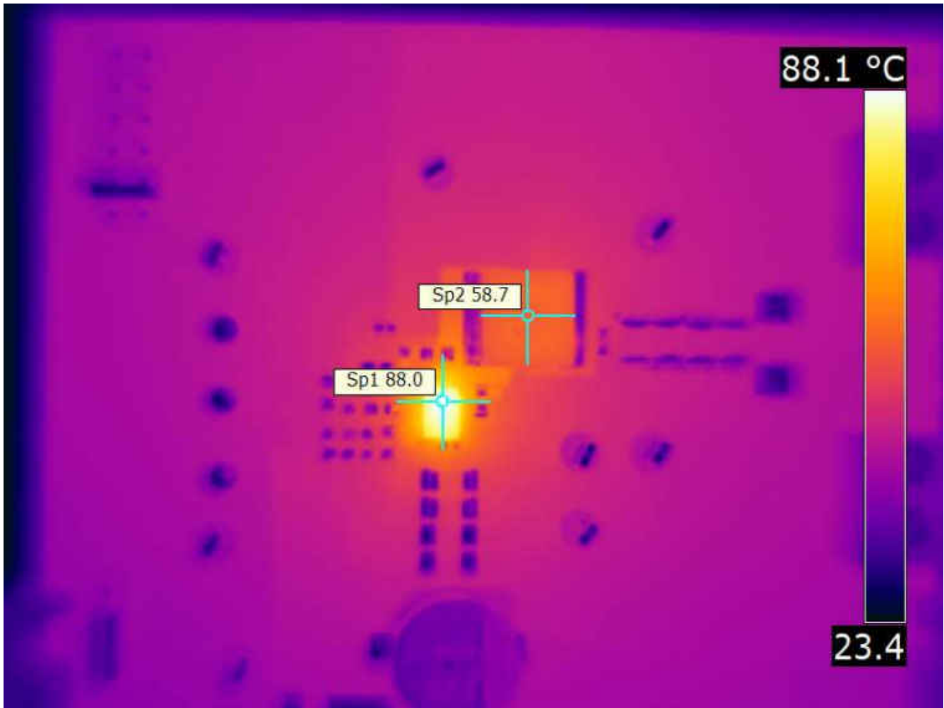
图 8-32. Thermal Image At 25^{\circ}\text{C} Ambient
