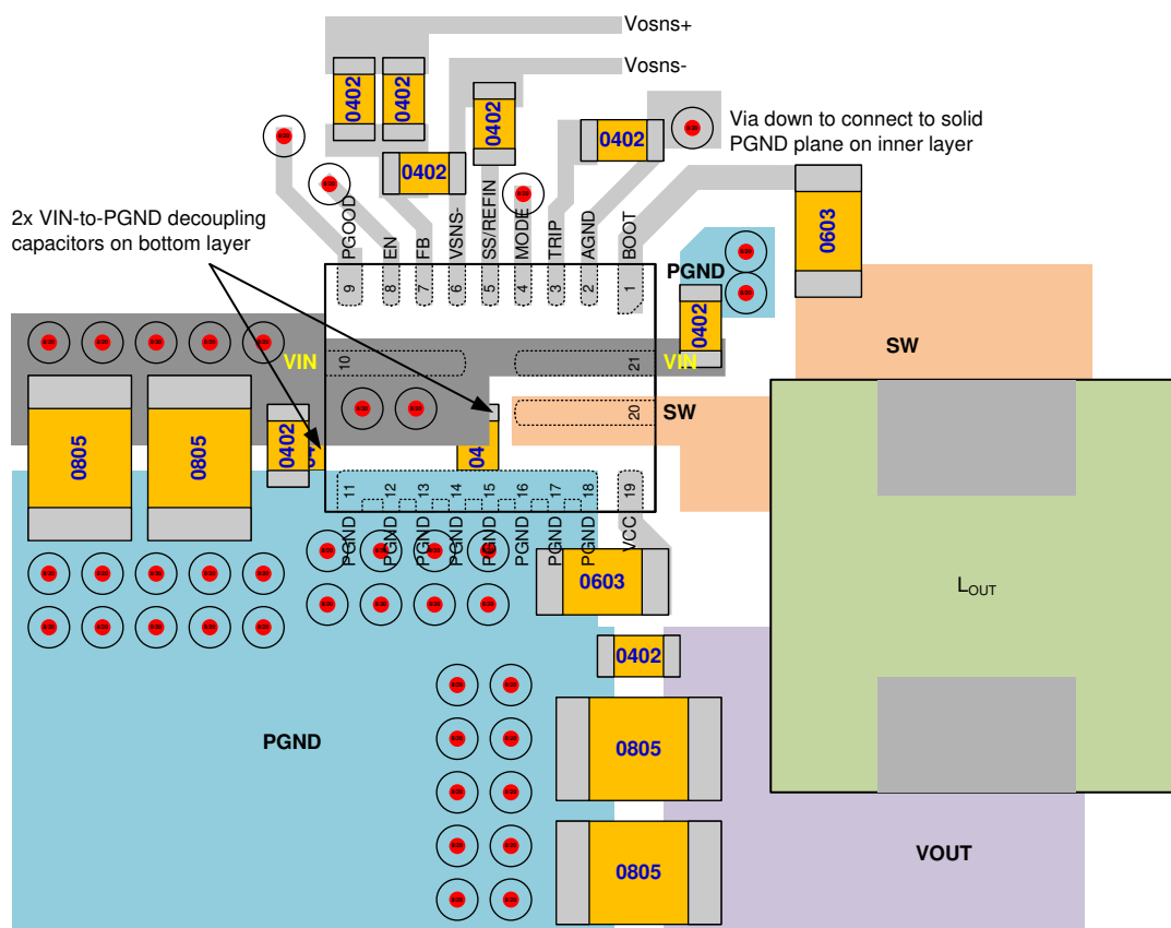
图 8-31. Layout Recommendation
