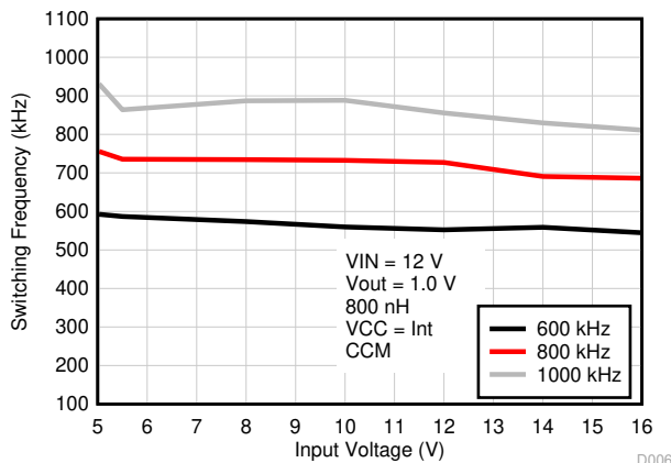
图 8-6. Switching Frequency vs Input Voltage
