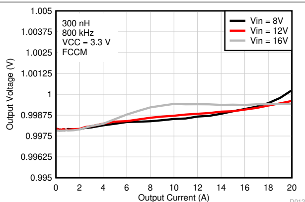
图 8-10. Output Voltage vs Output Current, VCC = 3.3-V External Bias
