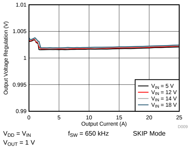
Figure 22. Output Voltage Regulation vs Output Current
