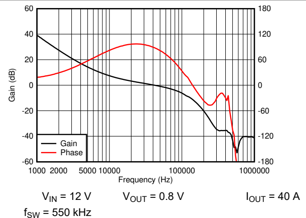
图 8-15. Total-Loop Bode Plot
