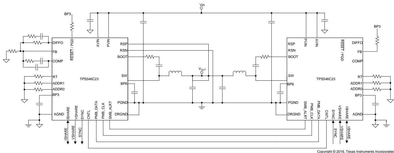
图 23. 2-Phase Application
