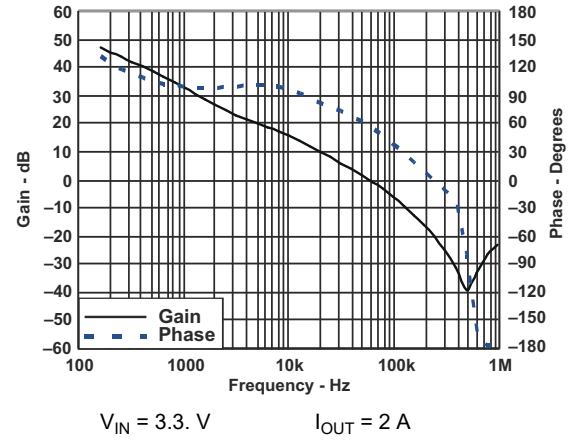
图 8-9. Closed-Loop Response
