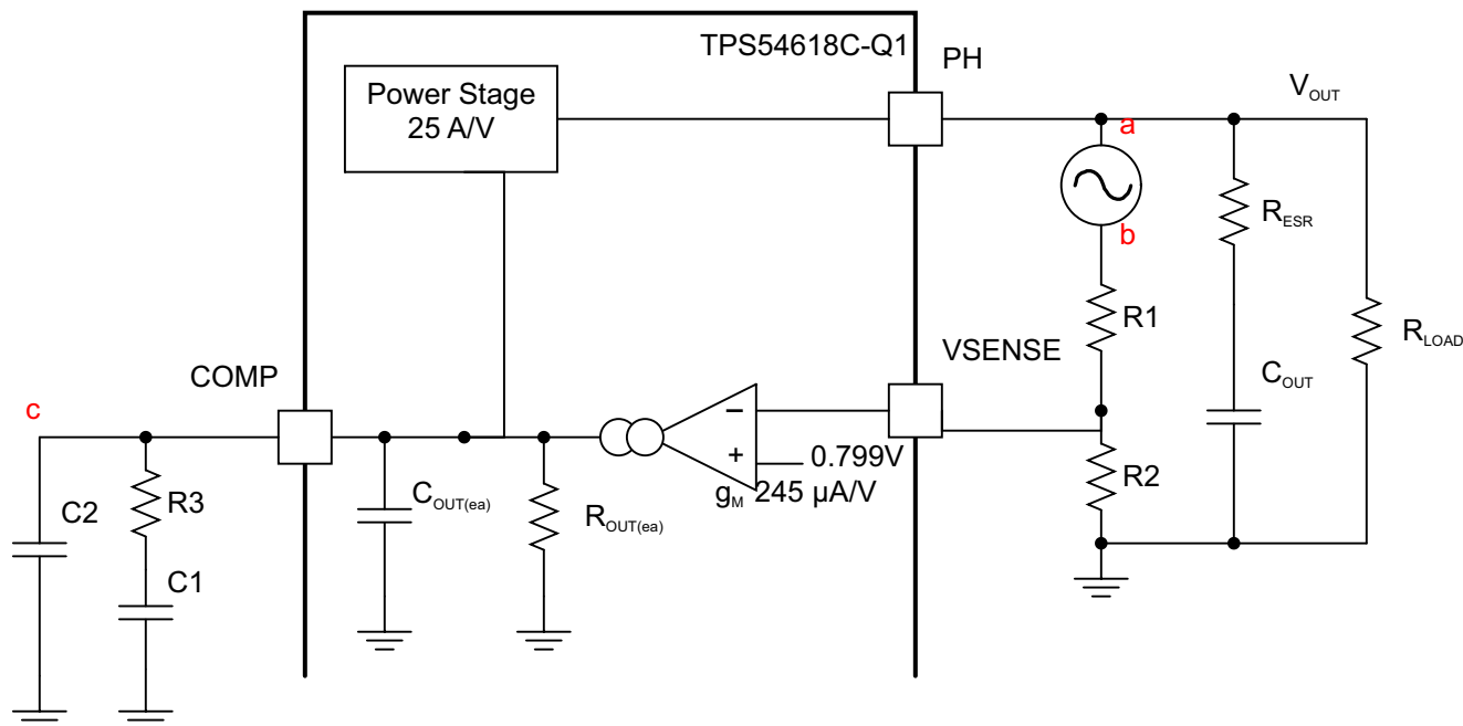
图 7-11. Small Signal Model for Loop Response
