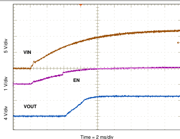
图 8-8. Start-up With VIN
