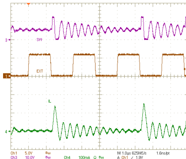
图 7-15. Plot of Synchronizing in Eco-mode
