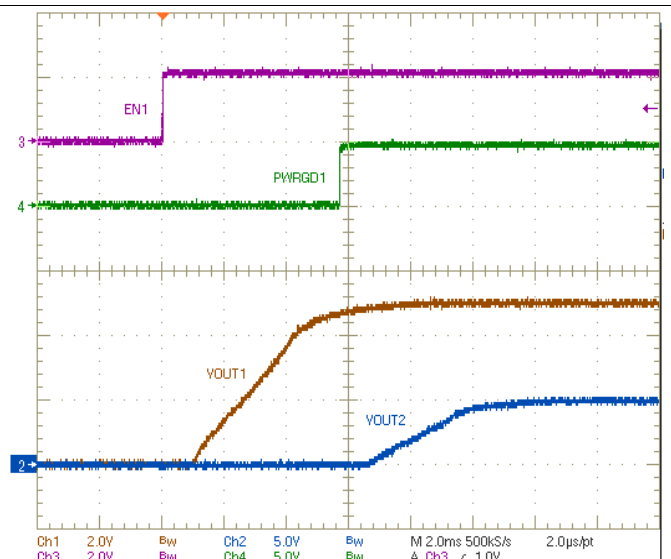
Figure 30. Sequential Startup using EN and PWRGD
