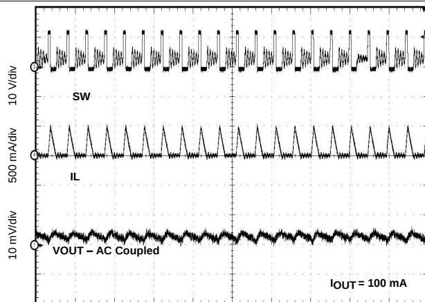
Figure 56. Output Ripple DCM
