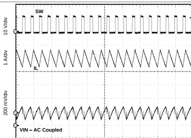
Figure 58. Input Ripple CCM
