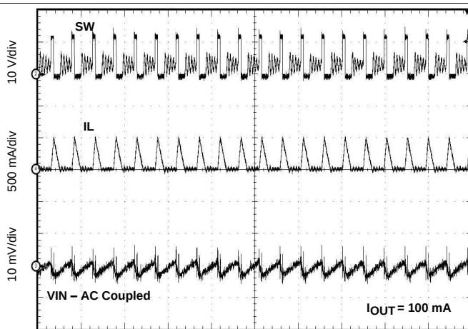
Figure 59. Input Ripple DCM
