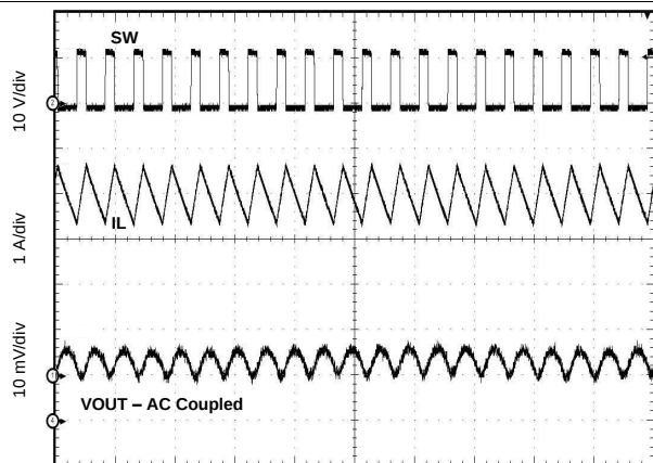
Figure 55. Output Ripple CCM
