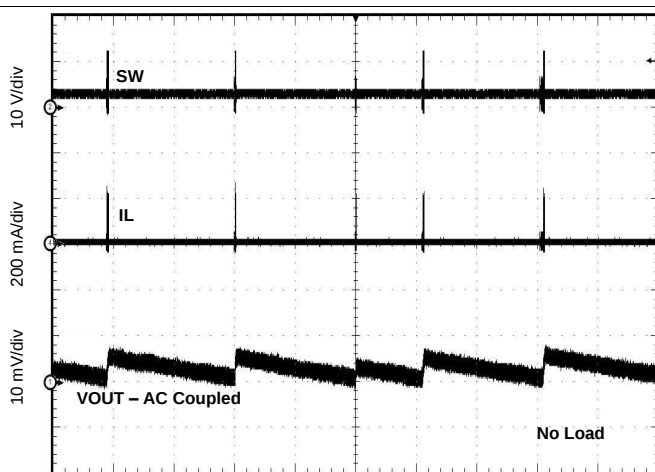
Figure 57. Output Ripple PSM
