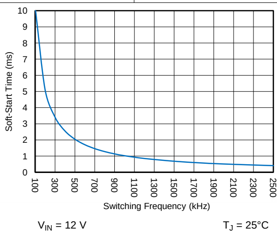
Figure 21. Soft-Start Time vs Switching Frequency
