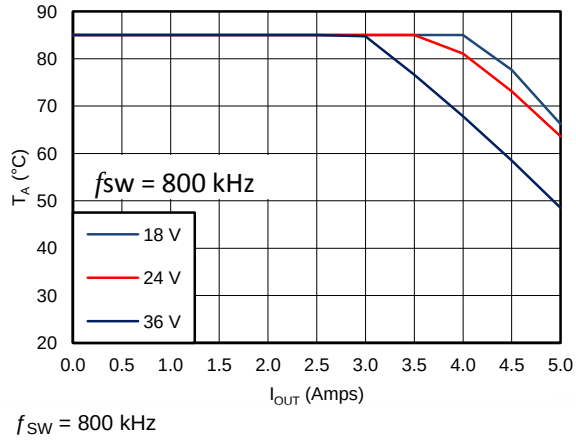
Figure 35. 12-V Outputs
