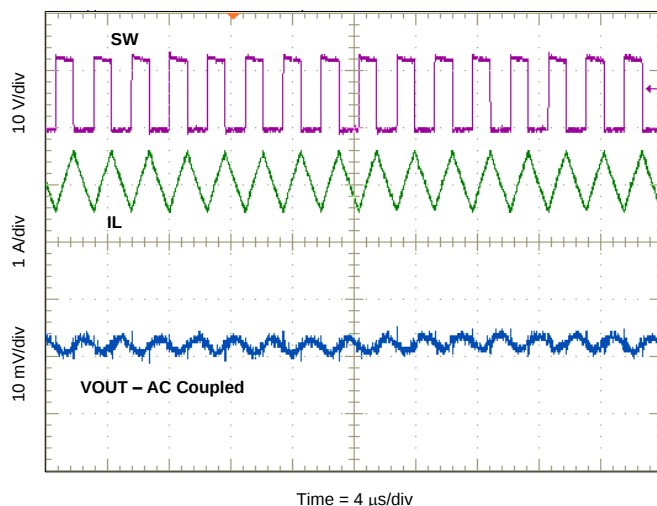
Figure 39. Output Ripple CCM
