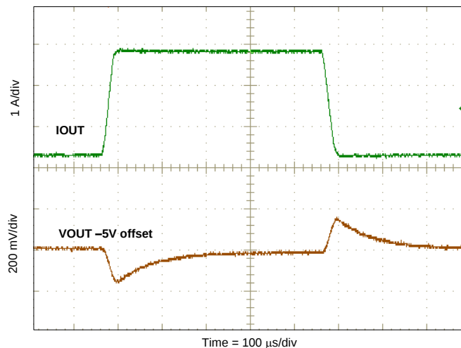
Figure 35. Load Transient
