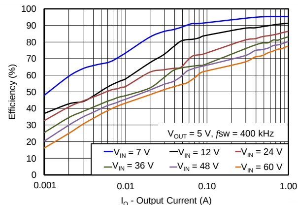
Figure 48. Light Load Efficiency
