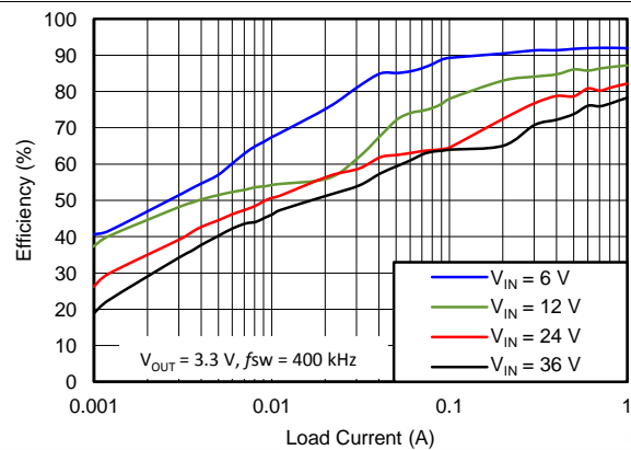
Figure 49. Light Load Efficiency
