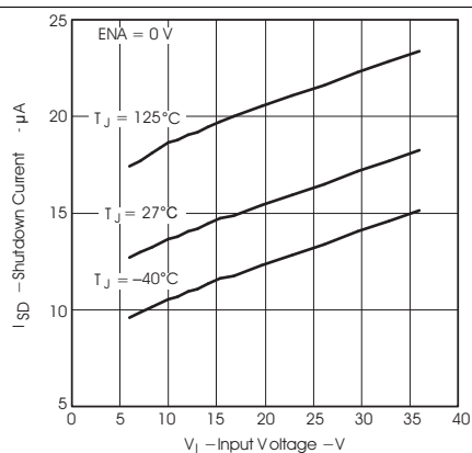
图 3. Shutdown Quiescent Current vs input Voltage
