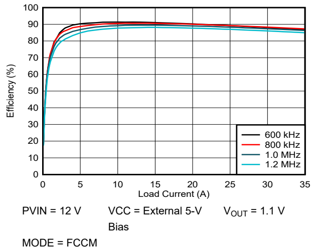
图 6-3. Efficiency vs Output Current
