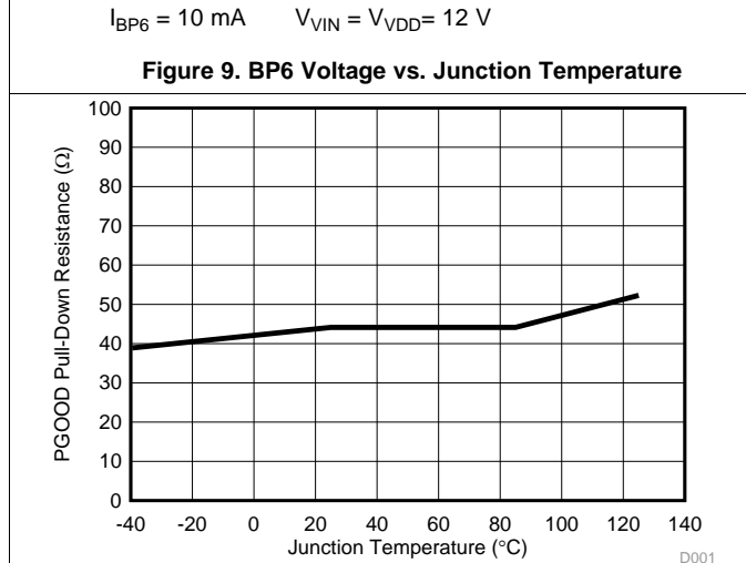
Figure 11. PGOOD Pull-Down Resistance vs. Junction Temperature
