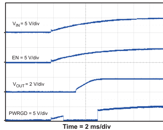
Figure 41. Power Up VOUT, VIN
