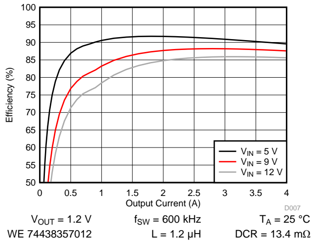
图 5. Efficiency for 1.2 V Output
