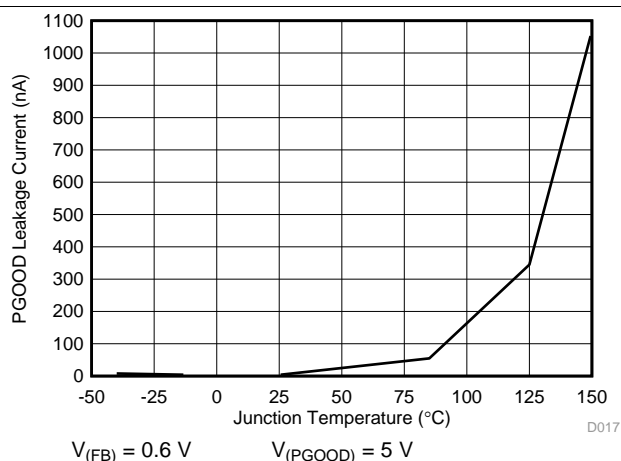
图 20. PGOOD Leakage Current vs Junction Temperature
