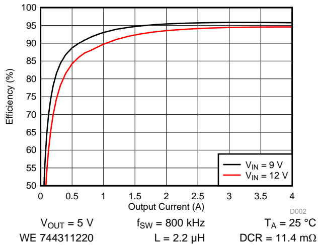
图 1. Efficiency for 5 V Output
