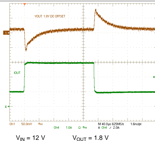
图 41. Transient Response
