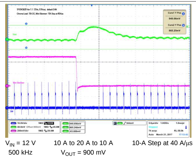
Figure 26. Transient Response When Load Steps Down
