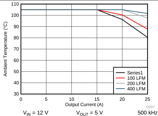
图 39. Safe Operating Area
