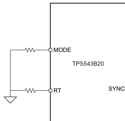
图 14. Stand-alone: RT Pin Sets the Switching Frequency
