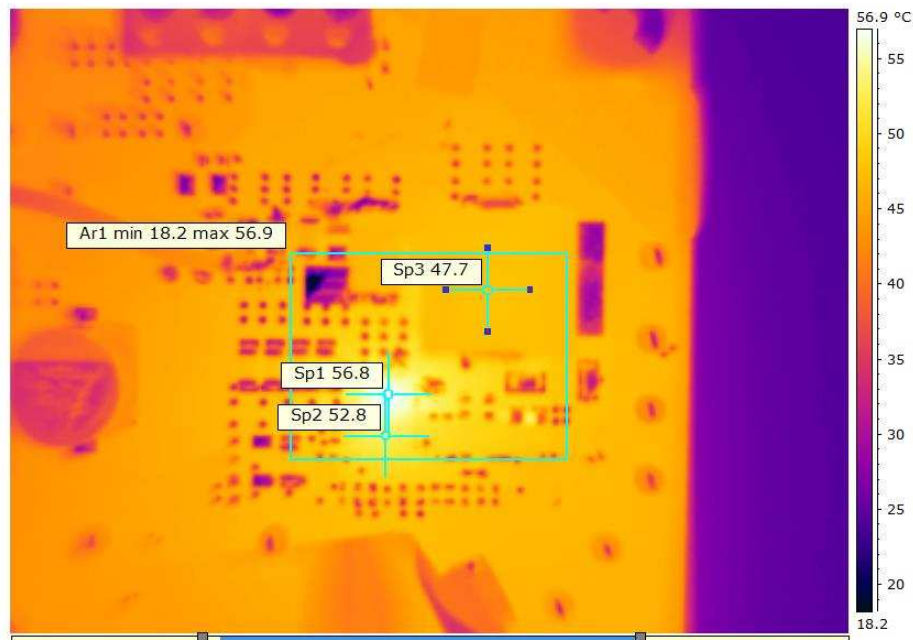
图 41. Thermal Image at 0.9-V Output at 12 VIN, 25-A Output, at 25°C Ambient
