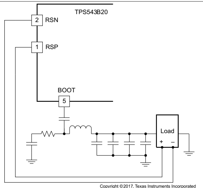
图 22. Remote Sensing Without Feedback Resistors
