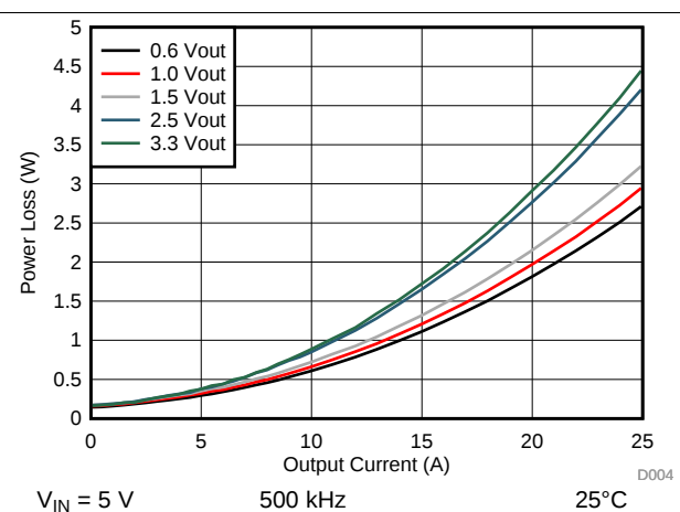
图 2. Power Loss vs Output Current
