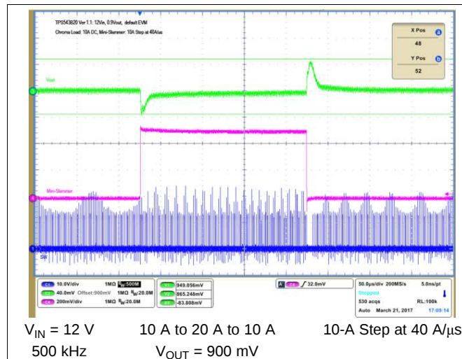
图 7. Output Voltage Transient Response
