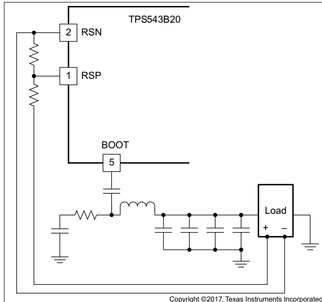
图 21. Remote Sensing With Feedback Resistors
