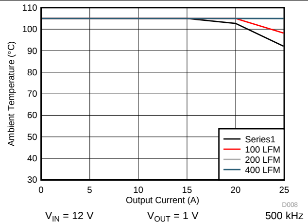
图 40. Safe Operating Area
