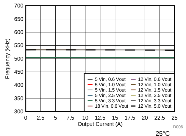
图 6. Switching Frequency vs Output Current
