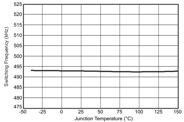
图 6-2. Frequency vs Temperature R_t = 400\text{ k}\Omega V_{IN} = 5\text{ V}
