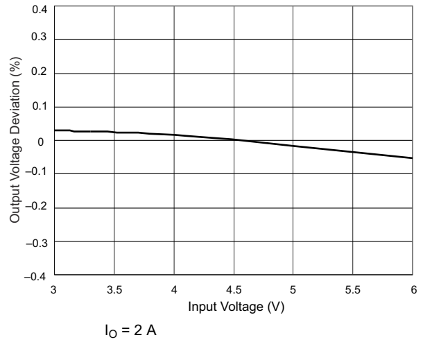
图 8-15. Regulation vs Input Voltage
