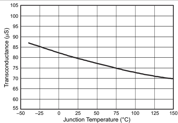
图 6-8. Transconductance (Slow Start) vs Junction Temperature
