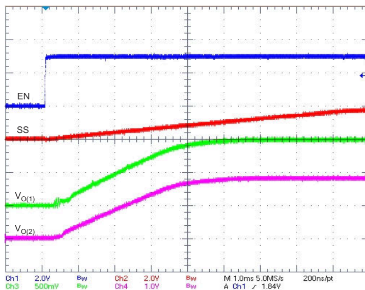
图 7-6. Ratiometric Start-Up With V_{O(1)} Leading V_{O(2)}
