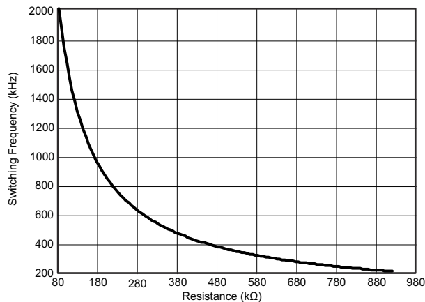
图 6-5. Switching Frequency vs R_T Resistance, Low-Frequency Range
