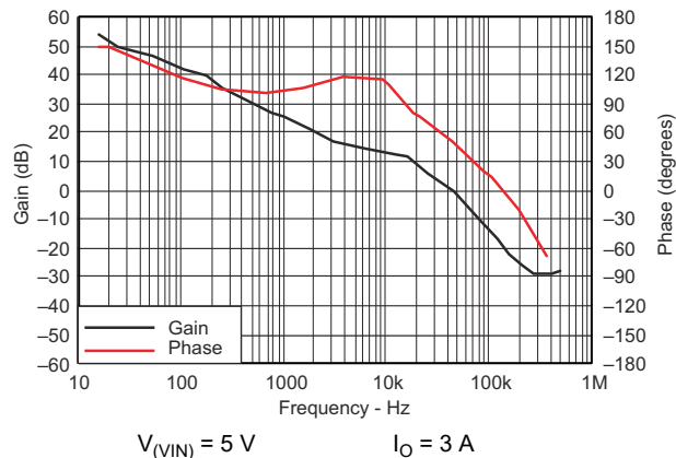
图 8-13. Closed-Loop Response
