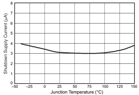
图 6-14. Shutdown Supply Current vs Temperature
