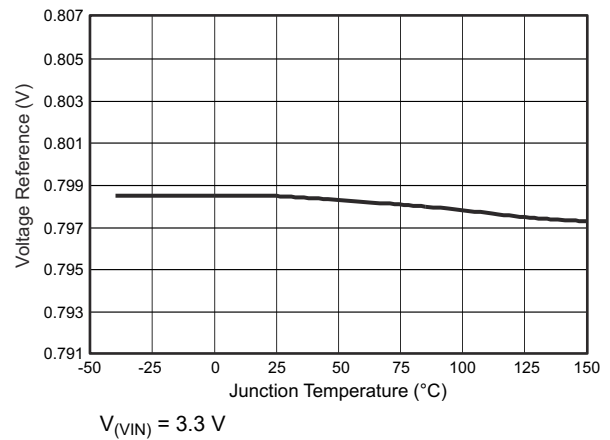
图 6-4. Voltage Reference vs Temperature V_{IN} = 3.3\text{ V}
