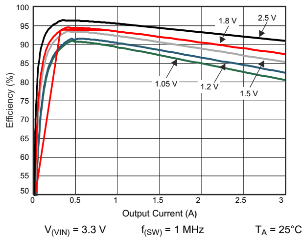
图 8-4. Efficiency vs Load Current
