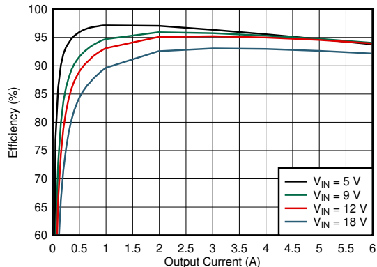
图 8-31. Efficiency
