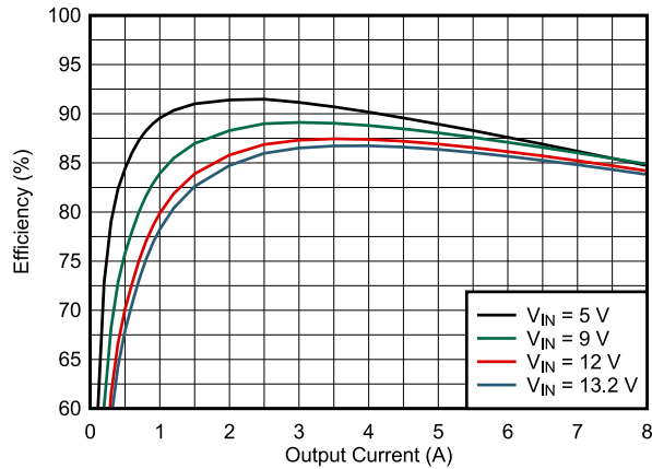
图 8-24. Efficiency
