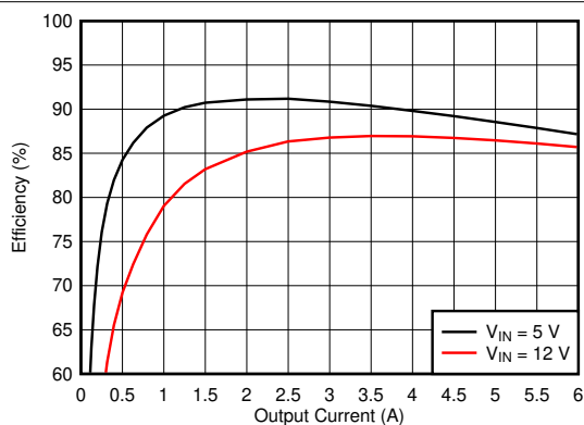
图 8-24. Efficiency
