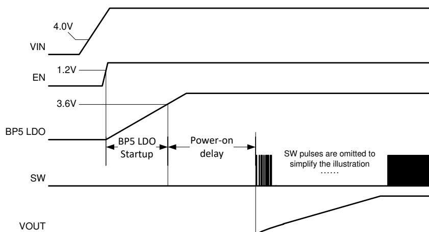
图 7-1. Start-up Sequence
