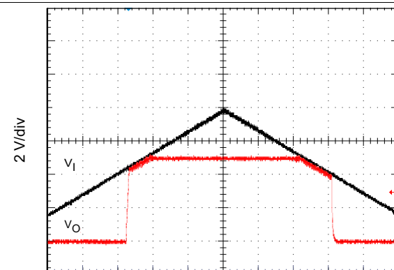
I_O = 1 \text{ A} EN floating Time = 40 \mu\text{s}/\text{div}
