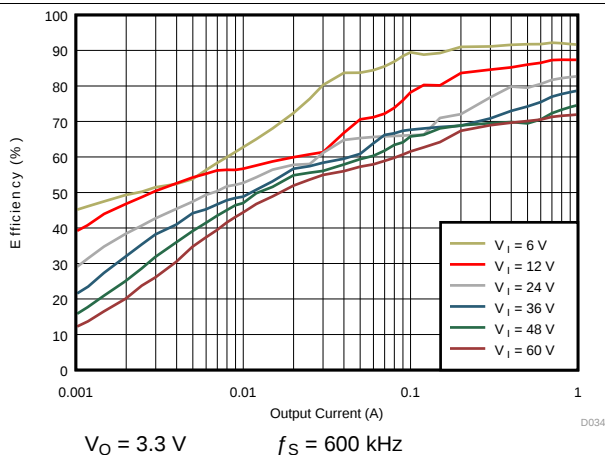
Figure 62. Light-Load Efficiency
