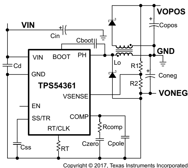
Figure 67. TPS54361 Split Rail Power Supply Based on the Application Note, SLVA369
