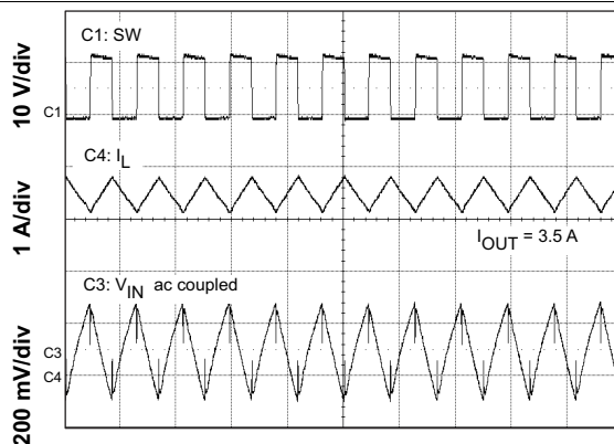
Time = 2 μs/div Figure 54. Input Ripple CCM
