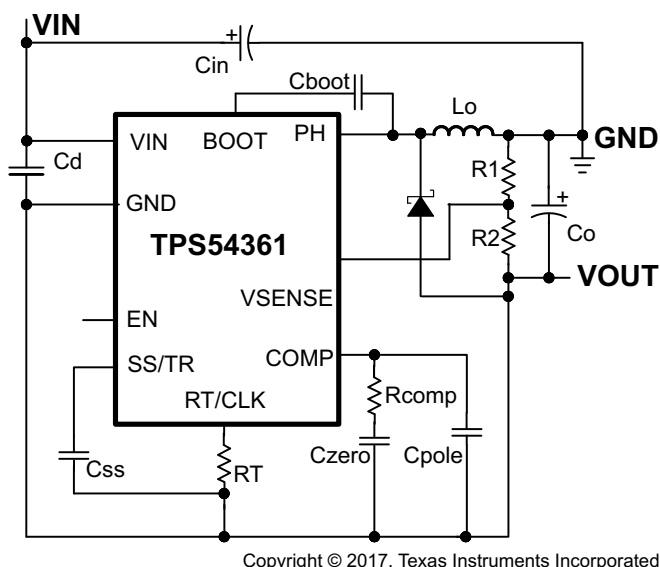
Figure 66. TPS54361 Inverting Power Supply Based on the Application Note, SLVA317
