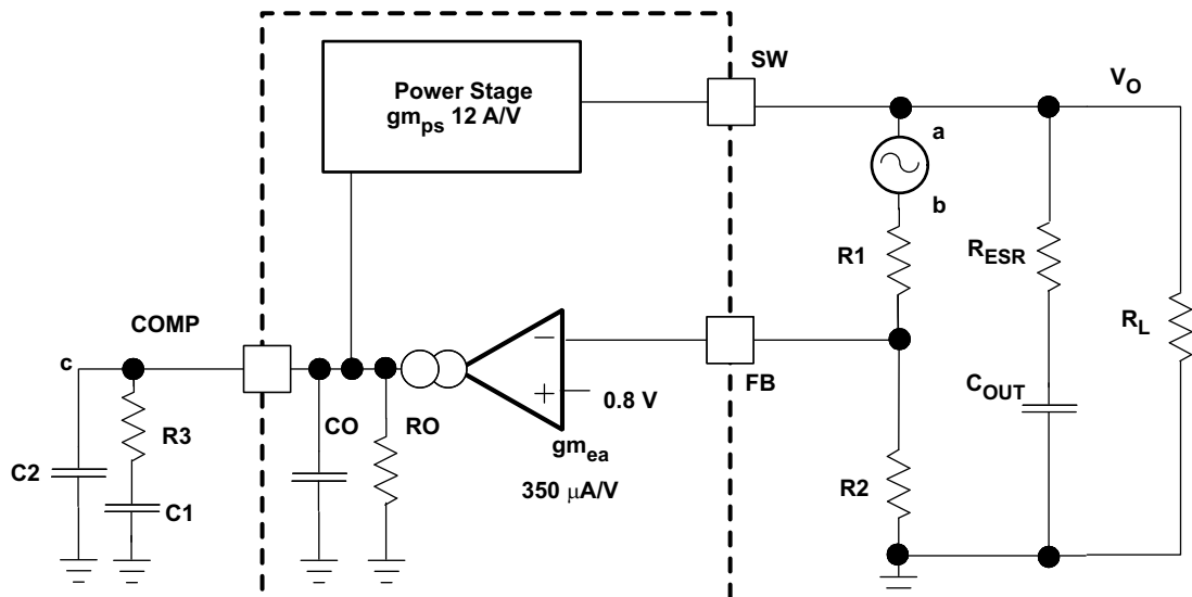
Figure 29. Small Signal Model For Loop Response
