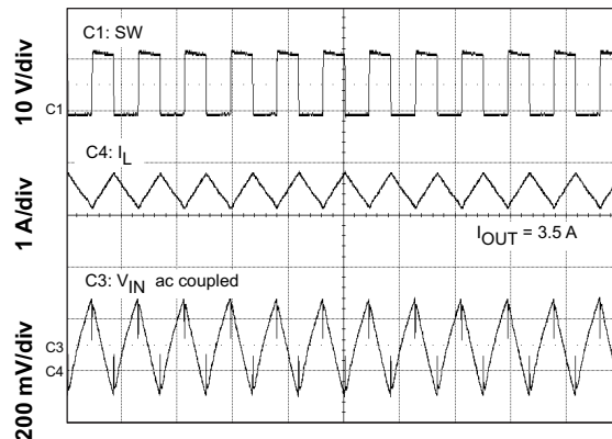
Figure 41. Input Ripple CCM
