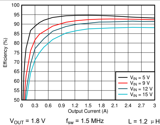
图 6-3. Efficiency vs Output Current
