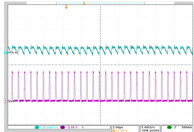
V_{IN} = 12\text{ V} I_{OUT} = 0\text{ A} 图 8-29. Input Ripple - No Load
