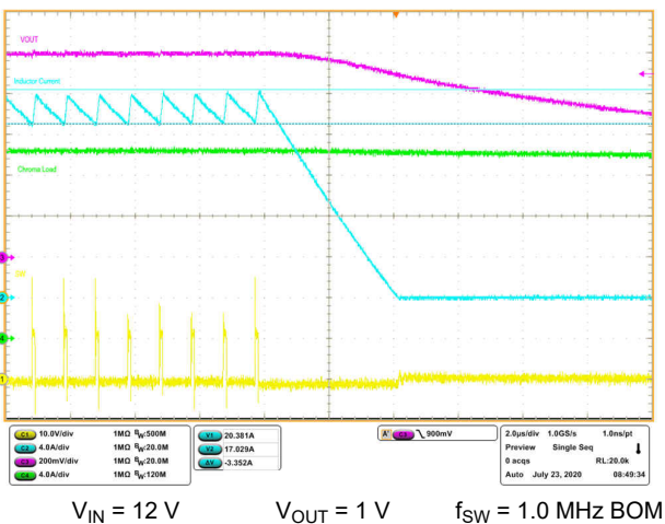
图 6-23. 20-A Overcurrent Protection by Electronic Load
