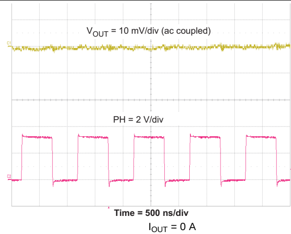
Figure 47. Output Ripple
