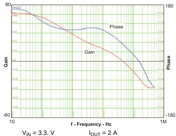
Figure 51. Closed Loop Response
