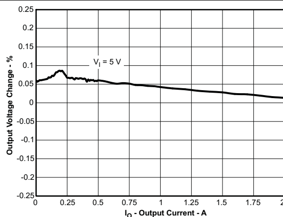
Figure 53. Load Regulation vs Load Current
