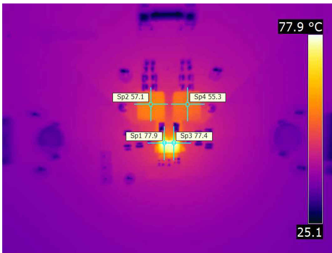
图 10-4. Thermal Image at 25°C Ambient - Dual Output Operation, f_{sw} = 1 \text{ MHz} , V_{IN} = 12 \text{ V} , V_{OUT1} = 1 \text{ V} , I_{OUT1} = 6 \text{ A} , L_1 = 560 \text{ nH} (3.3 mΩ Max), V_{OUT2} = 3.3 \text{ V} , I_{OUT2} = 6 \text{ A} , L_2 = 1.2 \text{ } \mu\text{H} (7.5 mΩ Max)
