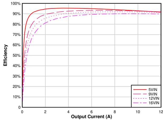
图 6-3. Efficiency vs Output Current, V_{OUT} = 3.3\text{ V} , F_{SW} = 1\text{ MHz}
