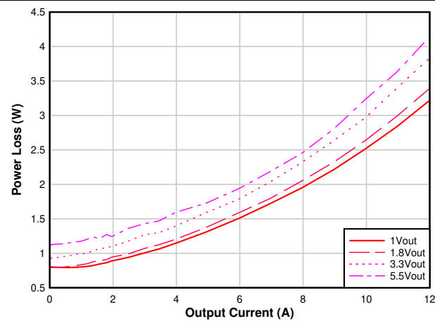
图 6-5. Power Dissipation vs Output Current, V_{IN} = 12\text{ V} , F_{SW} = 1\text{ MHz}
