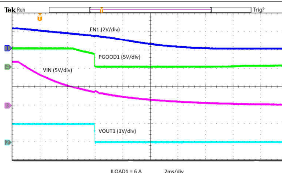
图 8-24. Power Down with V_{IN} V_{OUT1}
