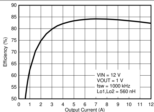
图 8-34. Efficiency
