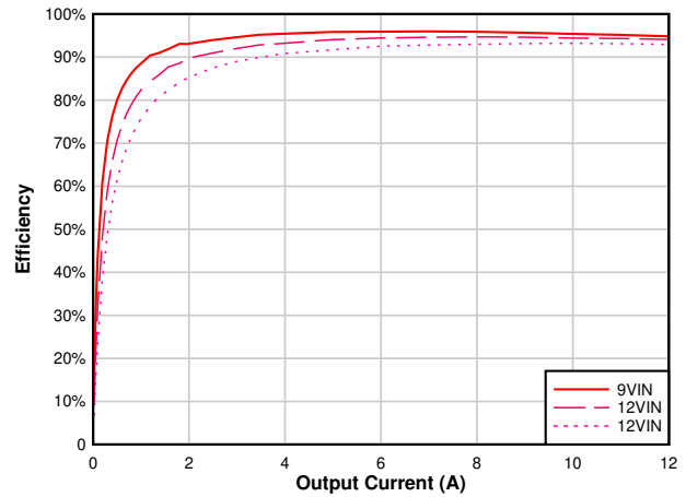
图 6-4. Efficiency vs Output Current, V_{OUT} = 5.5\text{ V} , F_{SW} = 1\text{ MHz}
