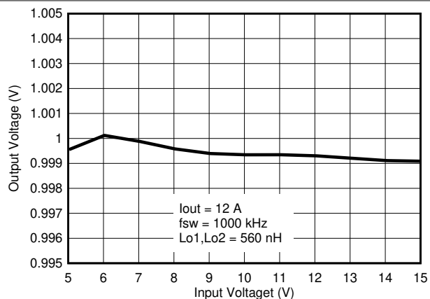
图 8-36. Line Regulation
