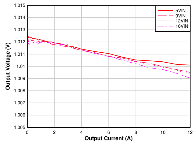
图 6-6. Output Voltage Regulation vs Output Current, V_{OUT} = 1.0\text{ V} , F_{SW} = 1\text{ MHz}
