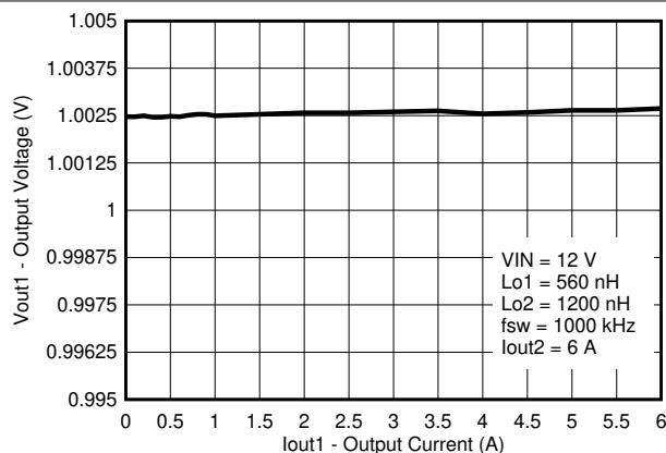
图 8-5. V_{OUT1} Load Regulation
