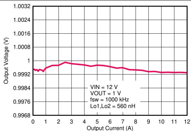
图 8-35. Load Regulation
