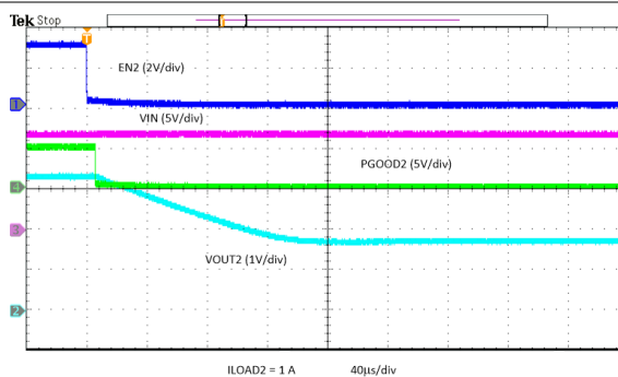
图 8-22. Power Down with EN 2 with Pre Bias
