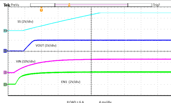
图 8-41. Power Up with V_{IN}
