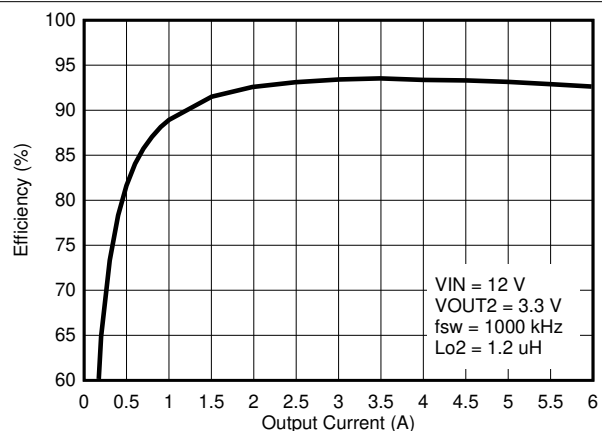
图 8-4. V_{OUT2} Efficiency
