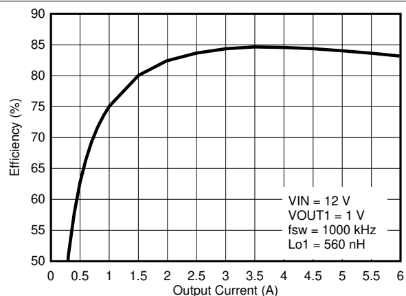
图 8-3. V_{OUT1} Efficiency
