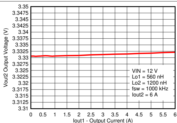
图 8-8. V_{OUT2} Cross Regulation
