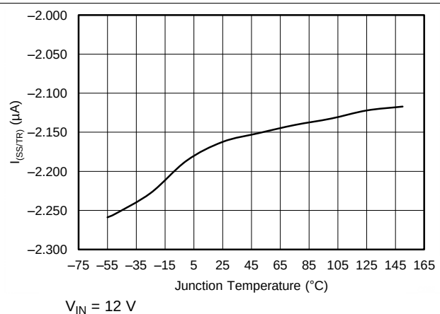
Figure 12. SS/TR Charge Current vs Junction Temperature
