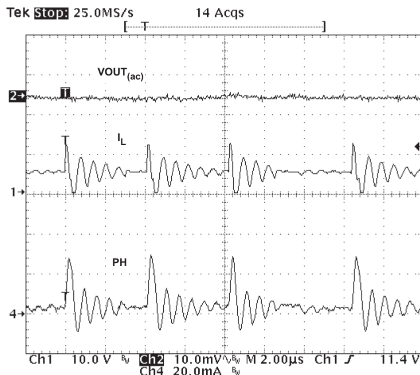
Figure 49. PSM Operation
