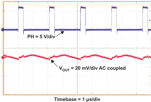
图 9-10. Output Voltage Ripple With Full Load
